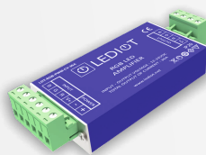
ldt-rgb-pwm-cv-36a
